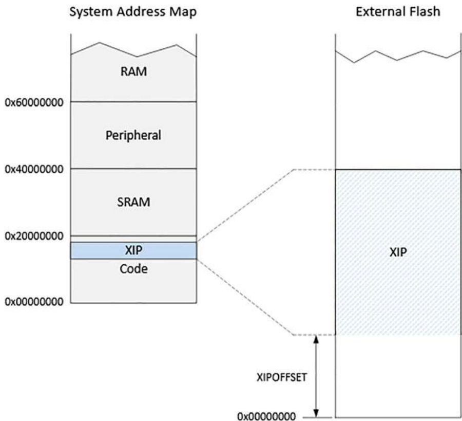
Figure 6-5. System Address Map showing mapping of XIP memory
