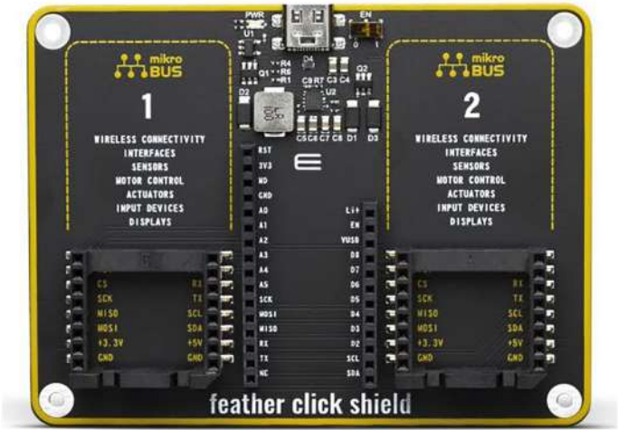
Figure 3-4. Mikroe feather click shield
