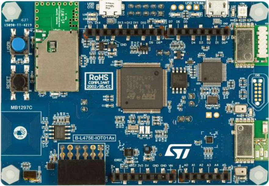
Figure 3-2. STM B-L475E-IOT01A Discovery kit
