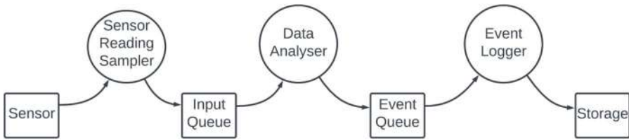
Figure 5-1. Common embedded system application scenario
