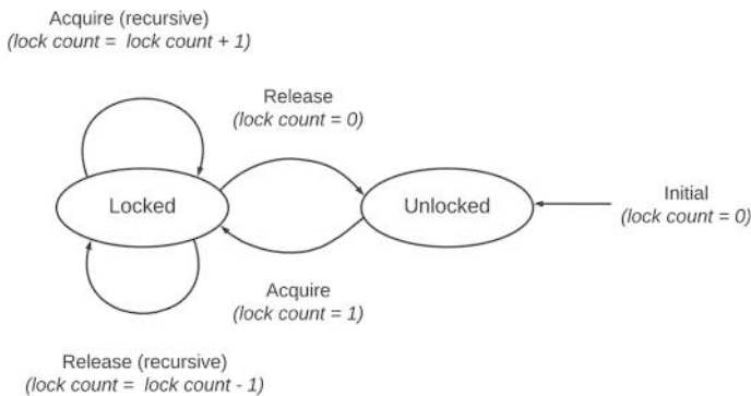
Figure 2-7. State machine for a recursive mutex
