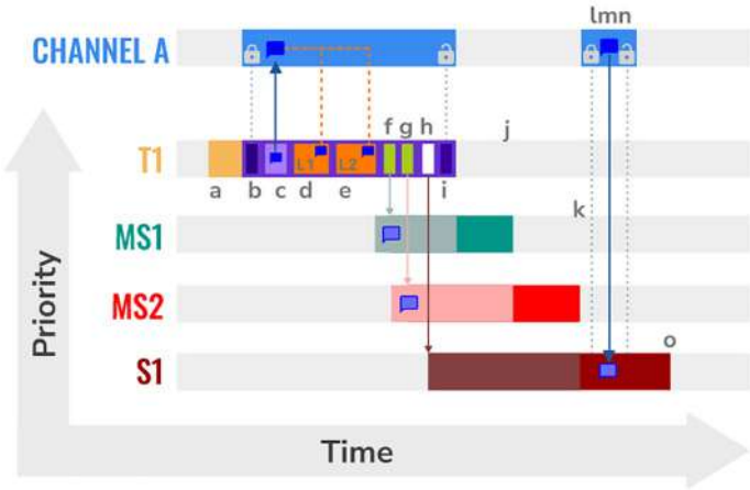
Figure 11-5. Example virtual distributed event dispatcher (VDED) scenario timing
