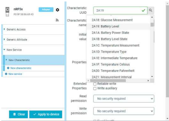
Figure 7-25. Selecting the Battery Level characteristic
