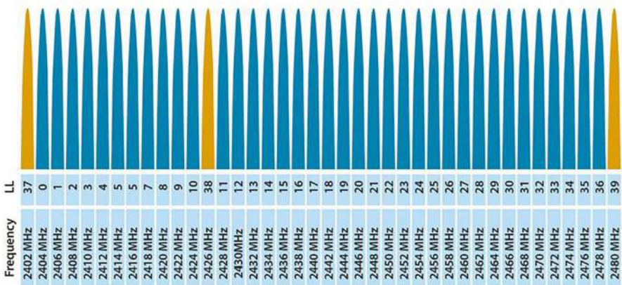
Figure 7-3. BLE RF channels, showing the Primary Advertising Channels (yellow)
