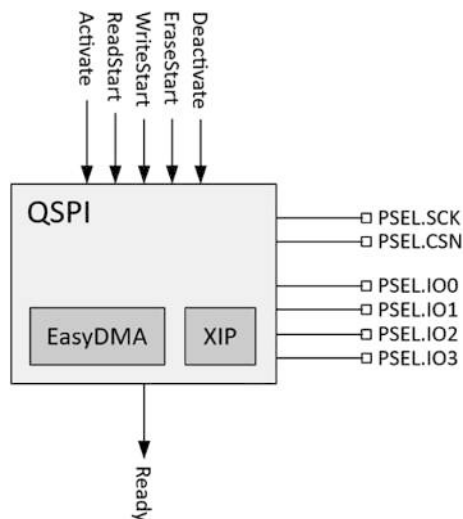
Figure 6-4. QSPI and Execute in Place (XIP)
