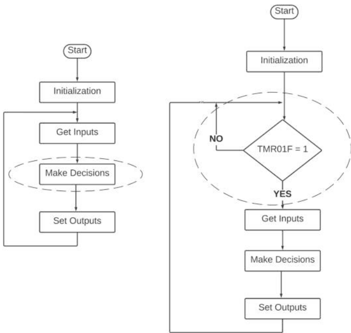
Figure 2-1. Big loop approach to embedded real time
