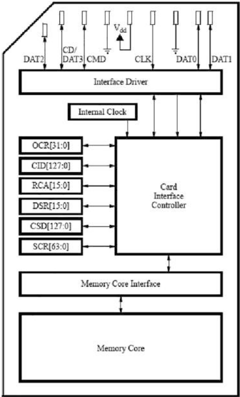
Figure 6-7. Schematic of architecture of SDC and MMC cards
