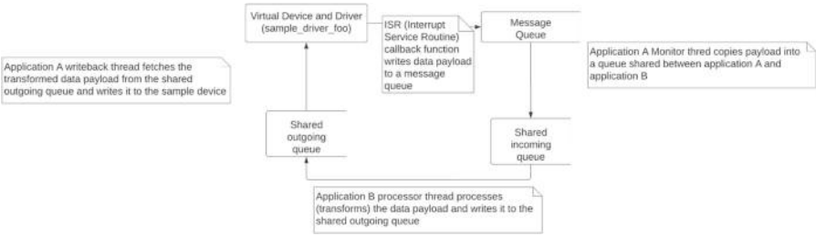
Figure 4-9. Zephyr producer-consumer example message processing flow
