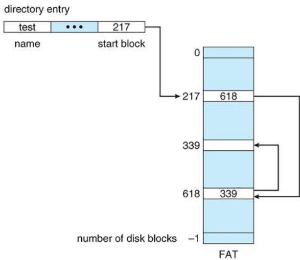
Figure 6-9. Block allocation in FatFs
