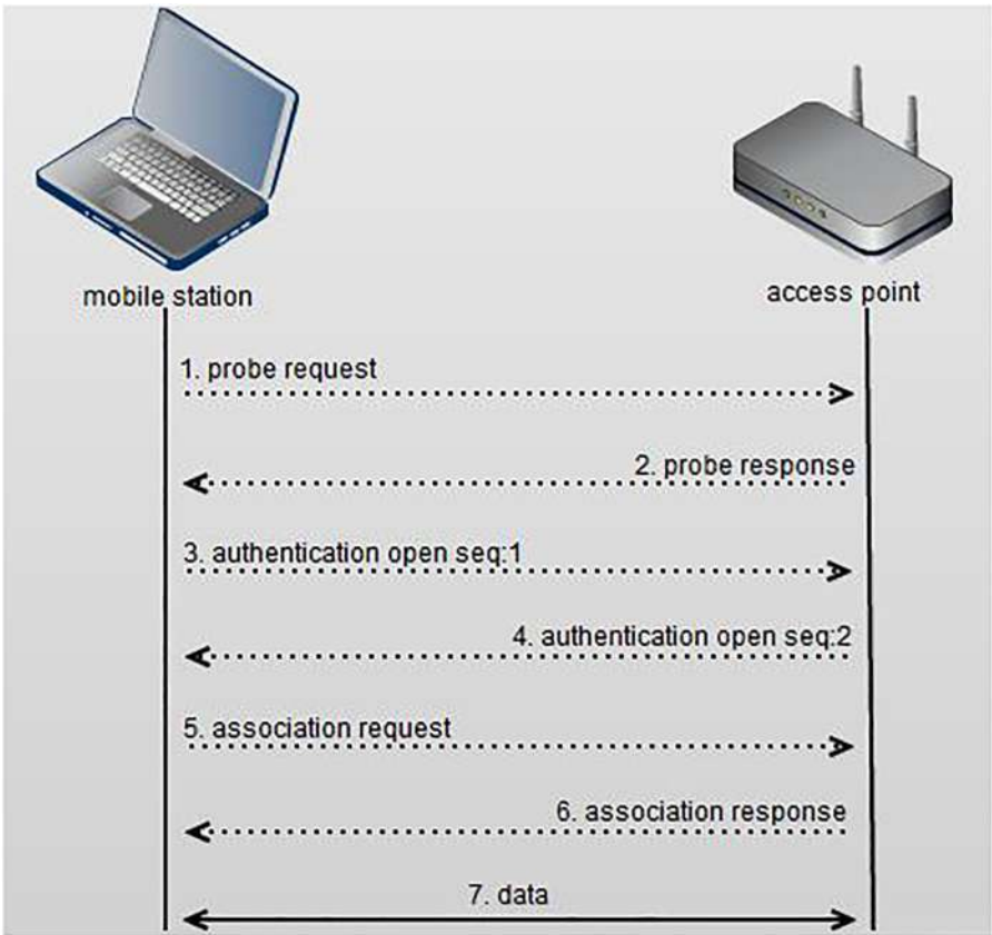
Figure 12-1. Authentication and Association Sequence Diagram
