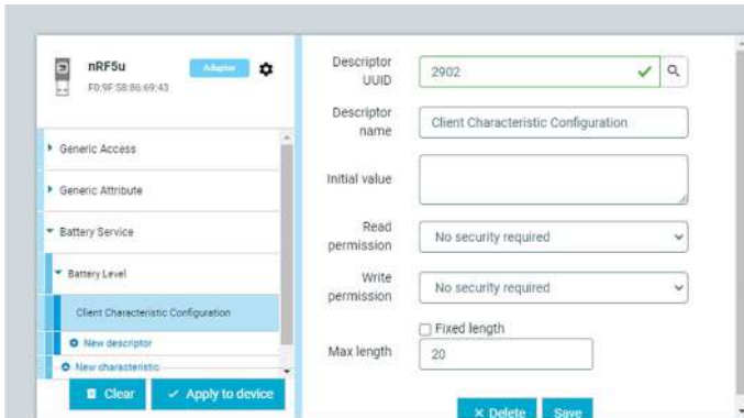
Figure 7-27. Configuring a Client Characteristic
