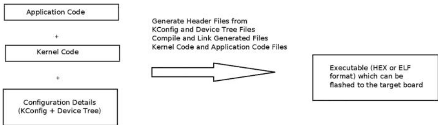
Figure 4-1. Generating an executable
