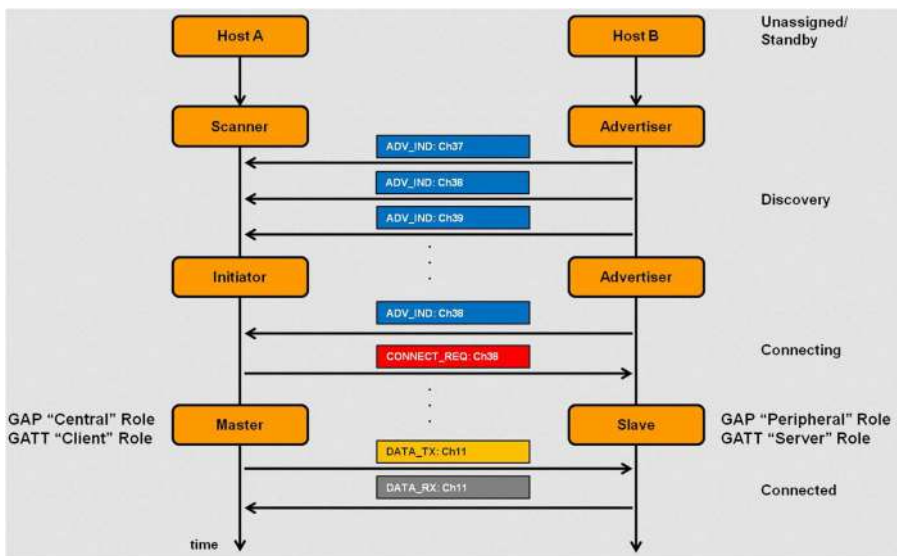
Figure 7-5. BLE unicast scenario sequence diagram
