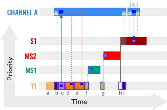
Figure 11-6. Example virtual distributed event dispatcher (VDED) scenario timing after priorities have been altered
