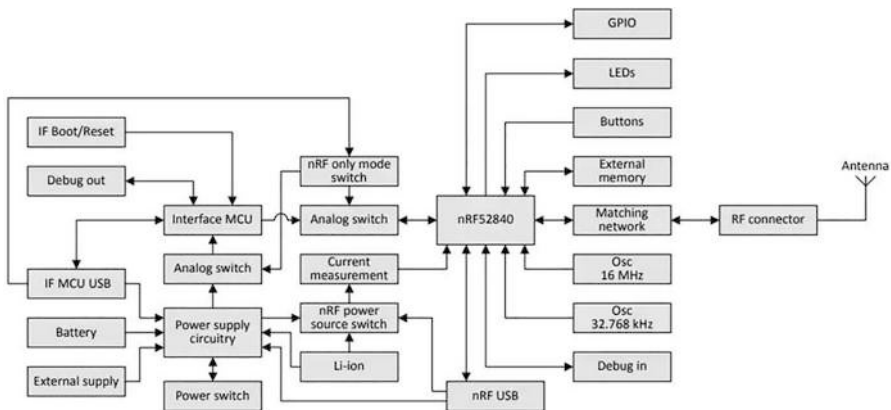
Figure 3-23. nRF52840 DK board schematic block diagram
