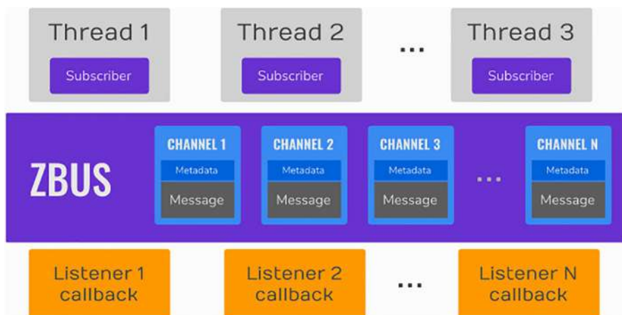
Figure 11-2. Schematic overview of the ZBus architecture
