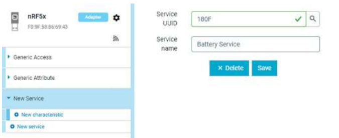
Figure 7-24. Configuring dongle to emulate the battery service
