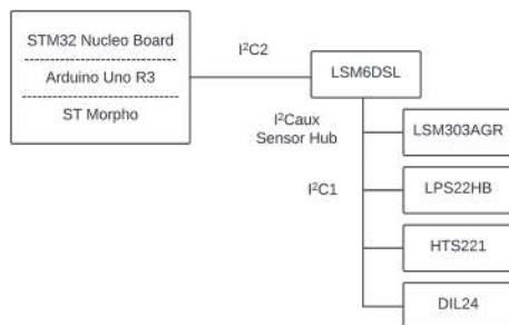
Figure 9-12. Schematic showing the I2C connections of the LSM6DSL device
