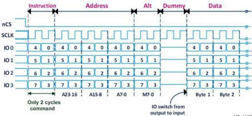
Figure 6-2. Quad-SPI clock cycle traces
