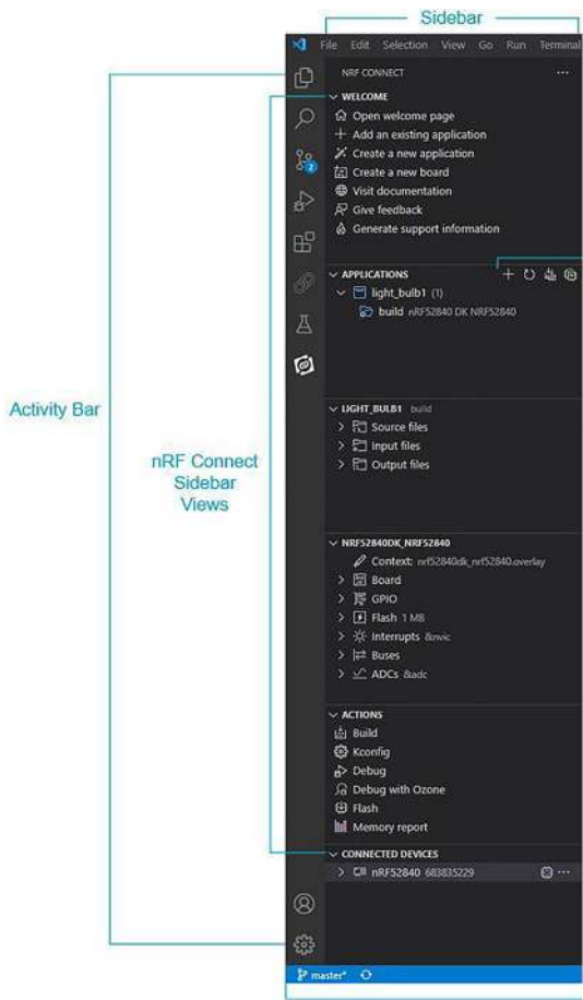
Figure 3-12. Activity Bar and nRF Connect Sidebar Views
