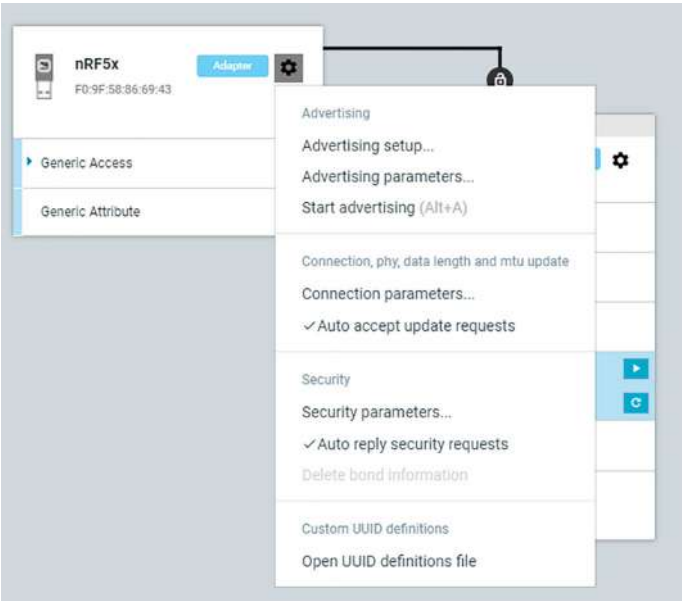
Figure 7-22. Advertising Menu showing Start advertising option
