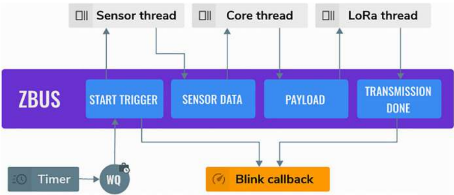
Figure 11-3. Example ZBus usage scenario
