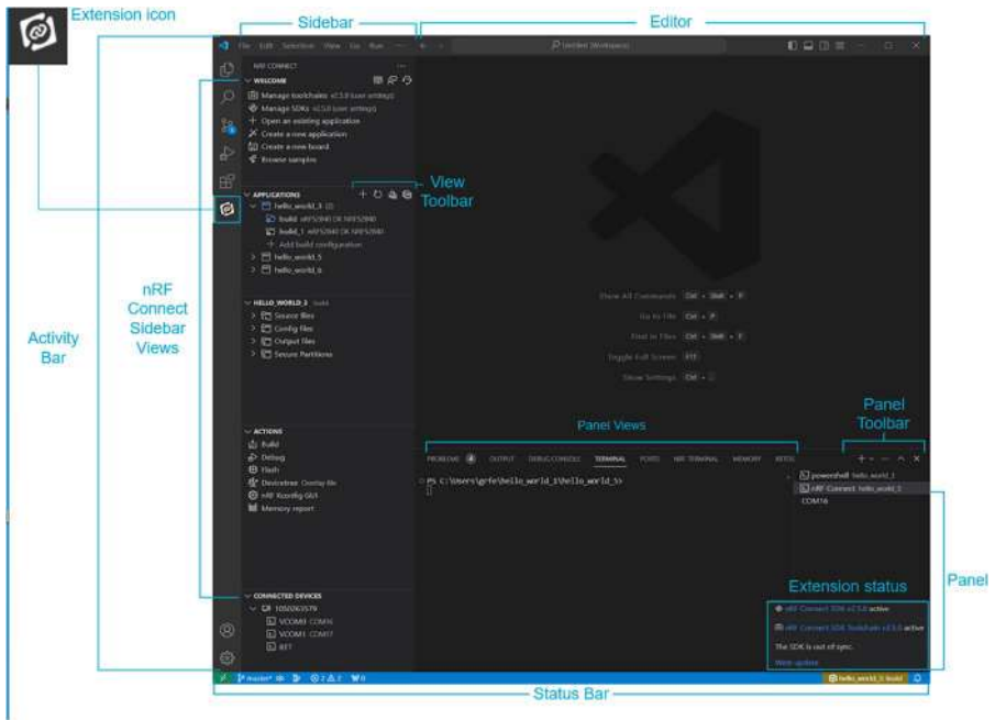
Figure 3-11. nRF Connect for VS Code Overview
