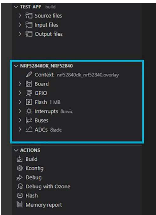
Figure 3-20. Devicetree View
