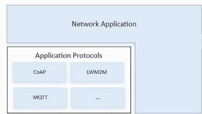
Figure 8-1. Network Application
