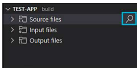
Figure 3-19. Details View
