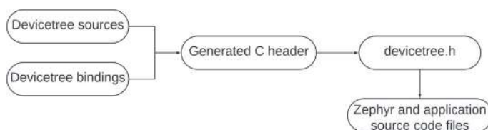
Figure 9-3. Generating devicetree.h
