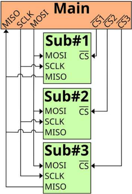
Figure 9-1. Simple SPI network schematic
