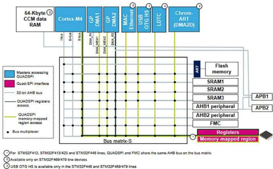
Figure 6-6. QSPI in STM32 processors
