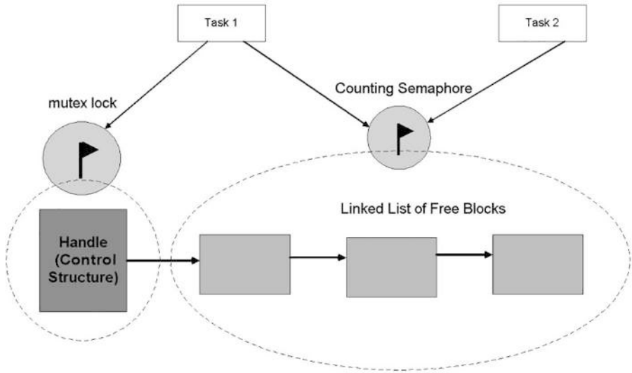
Figure 2-13. How to ensure atomic allocation of a memory block
