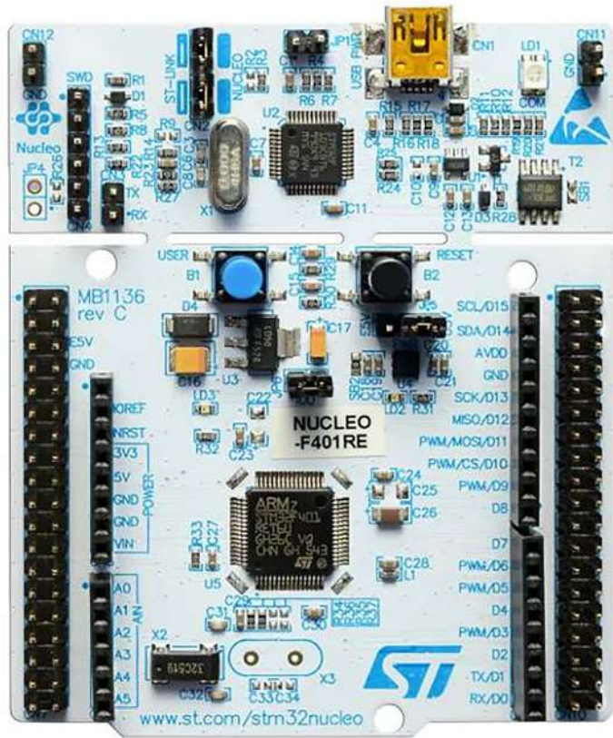
Figure 3-1. Nucleo-F401RE
