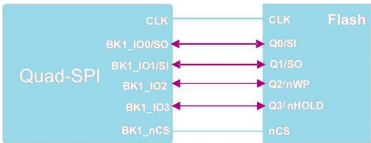
Figure 6-1. Typical Quad-SPI configuration
