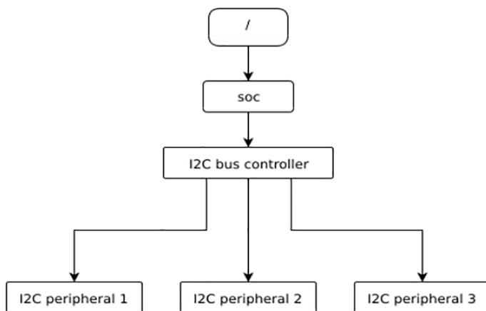
Figure 9-5. A devicetree fragment describing an on-chip I2C bus controller with three attached I2C peripherals
