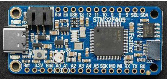
Figure 3-3. Adafruit Feather STM32F405 Express board
