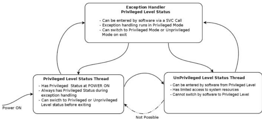
Figure 4-4. Transitions between privileged and unprivileged levels and exception handling
