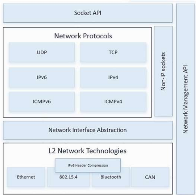
Figure 8-2. Network Protocols
