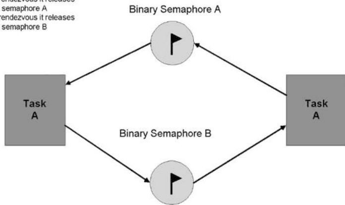
Figure 2-14. Basic rendezvous
