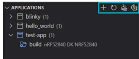
Figure 3-16. View Toolbar
