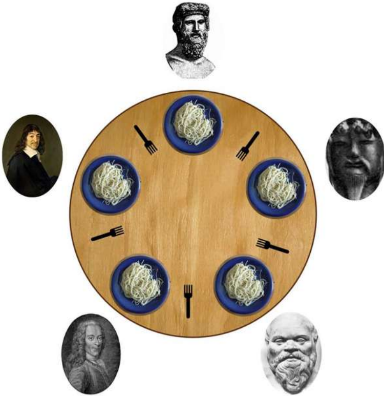
Figure 4-8. Dining philosophers
