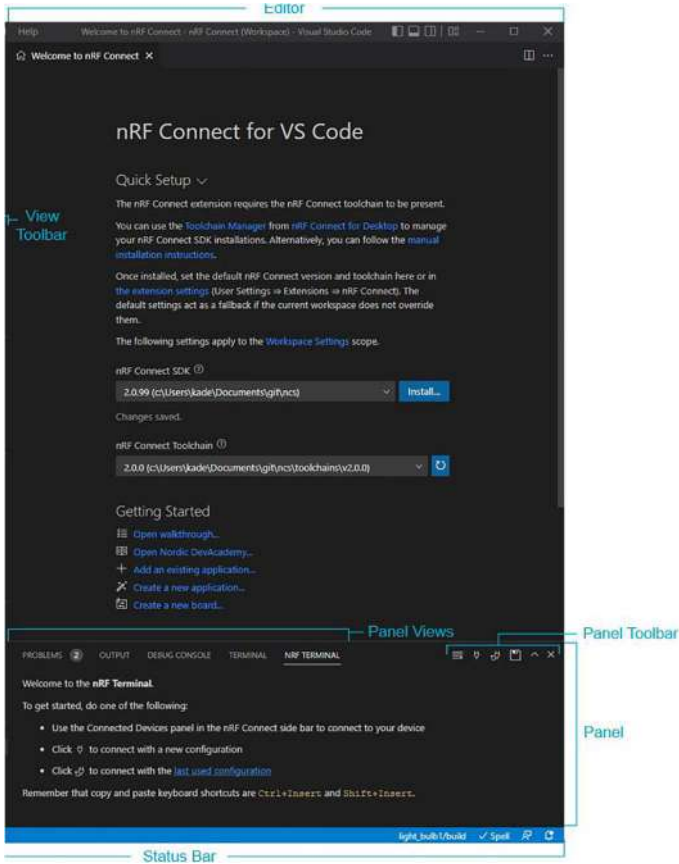
Figure 3-13. Editor Window, Panel Views, and Status Bar
