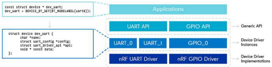
Figure 3-22. Zephyr device driver architecture
