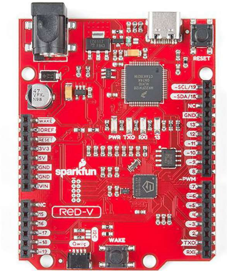
Figure 3-6. SparkFun’s RED-V SIFIVE RISC-V REDBOARD
