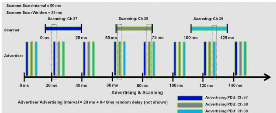
Figure 7-4. BLE link layer advertising and scanning
