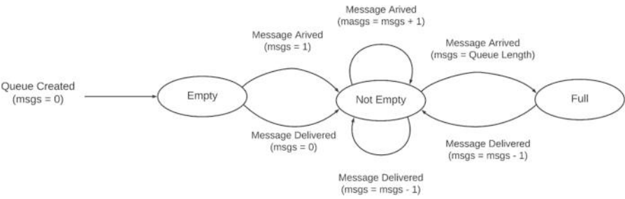
Figure 2-9. State machine for a message queue
