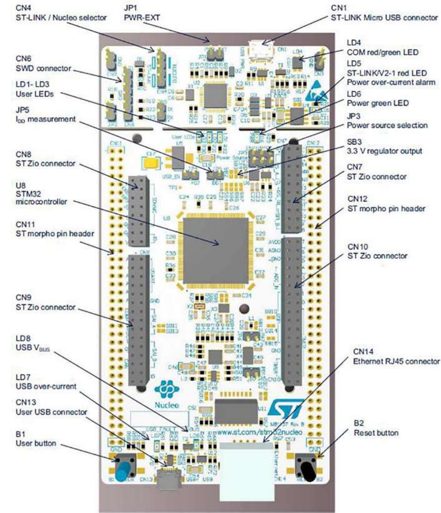
Figure 8-5. Nucleo-F767ZI Board layout
