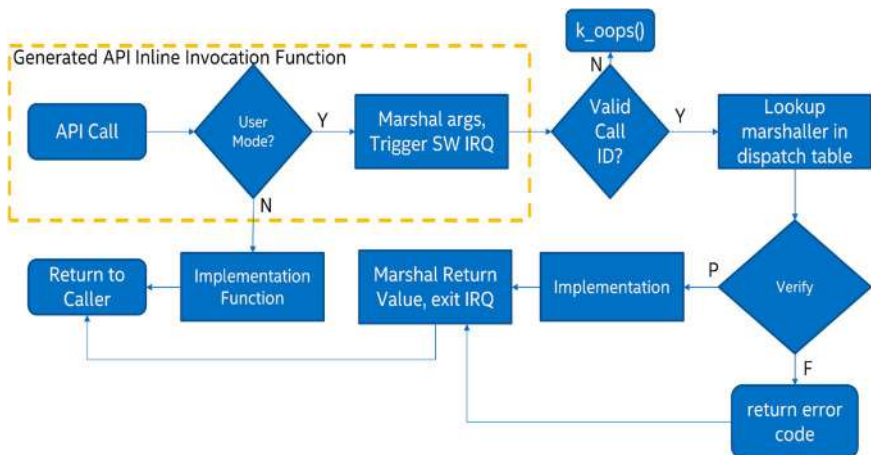
Figure 4-10. Zephyr RTOS system call execution flow
