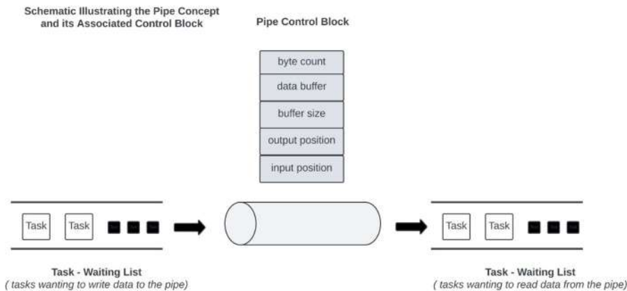
Figure 2-10. Schematic of a pipe and its associated control block
