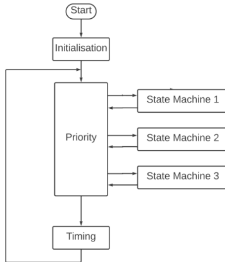
Figure 2-2. Incorporating priority-based multitasking into a big loop approach
