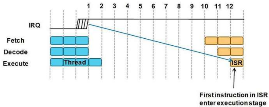
Figure 2-12. Interrupt latency of an ISR
