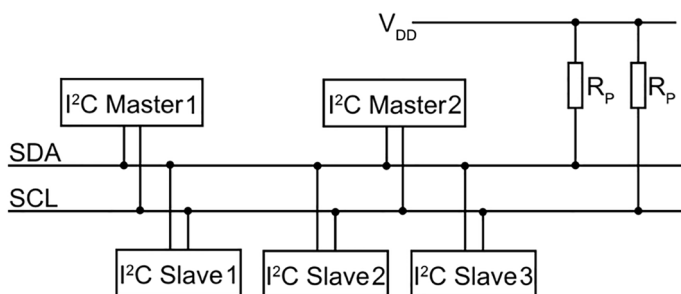
Figure 9-2. Simple I2C network schematic
