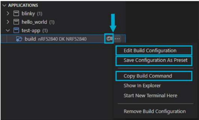
Figure 3-18. Build-specific actions
