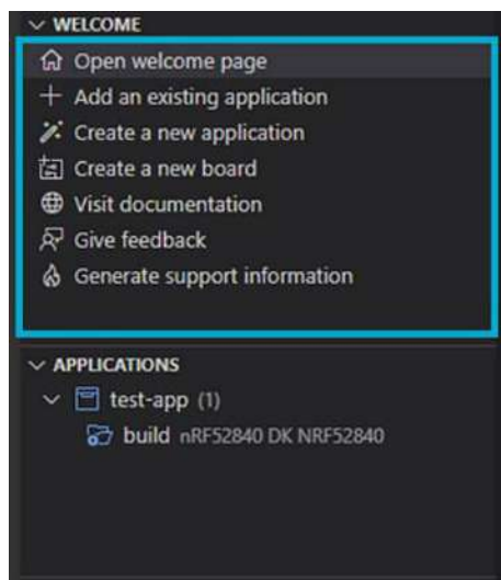
Figure 3-14. Welcome View
