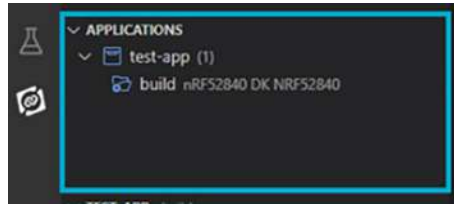
Figure 3-15. Applications View
