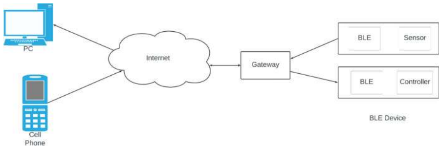
Figure 7-1. BLE sensor and BLE controller gateway connectivity to computer and mobile devices
